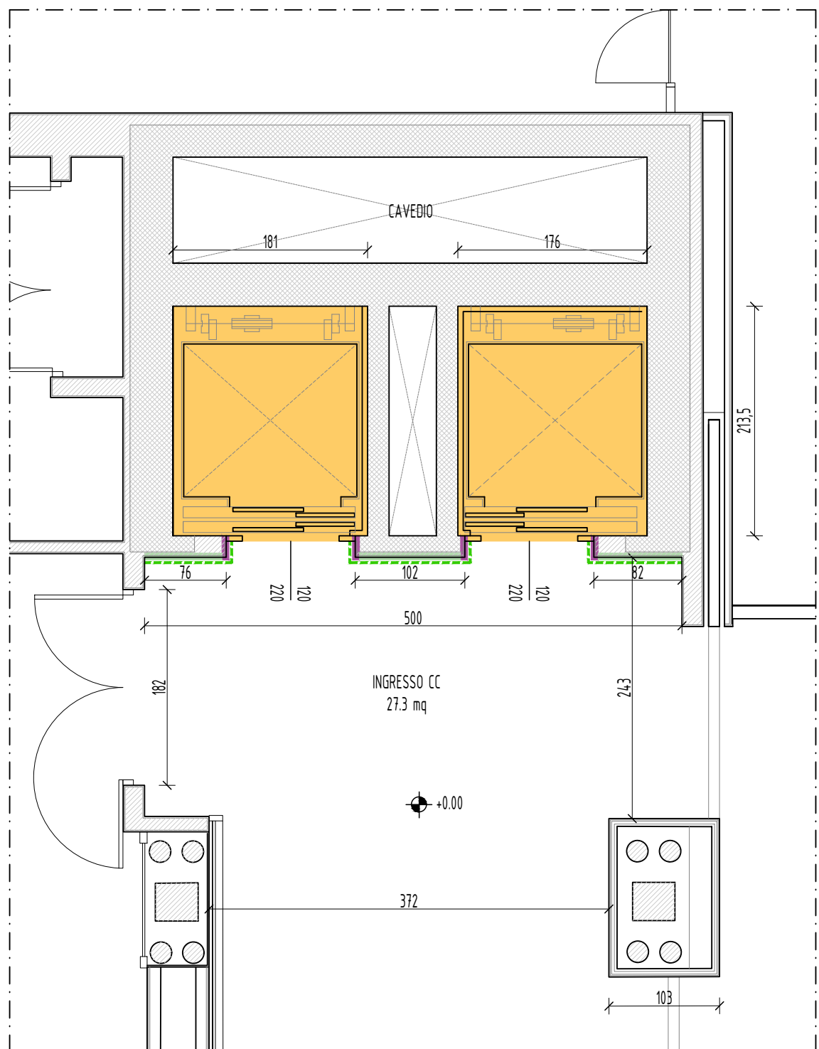
PIANO TERRA - 1:50
