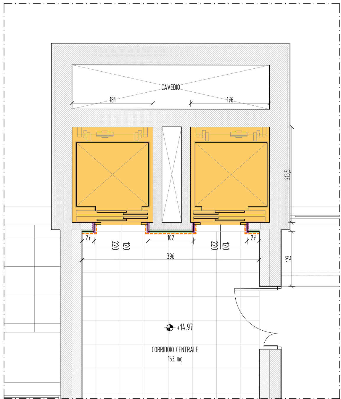
PIANO QUARTO - 1:50
