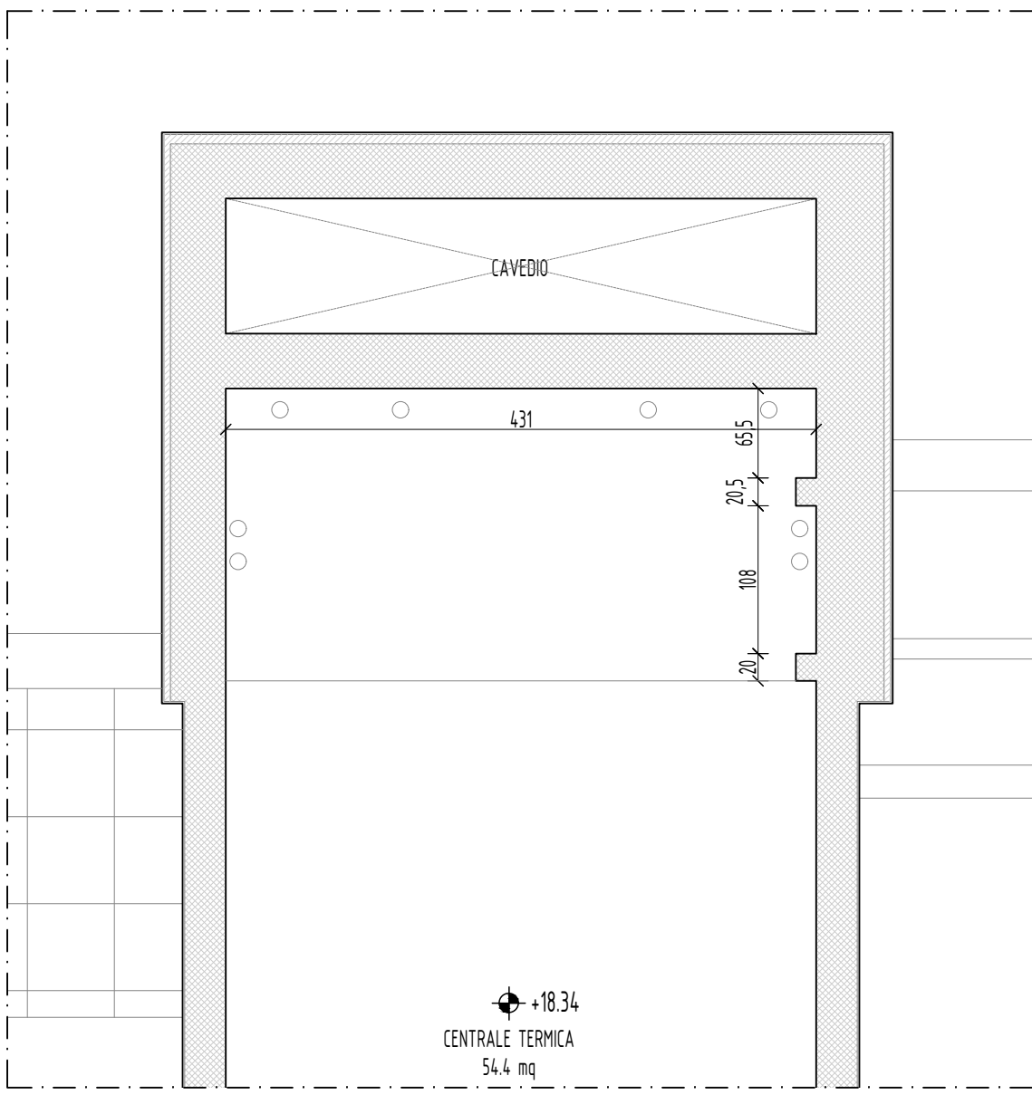
PIANO QUINTO - 1:50
